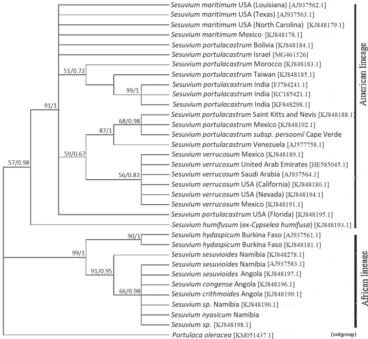
Figure 6. Phylogenetic relationships of perennial Sesuvium species from ML analysis of ITS sequences. The tree is drawn to scale, with branch lengths measured in the number of substitutions per site. ML bootstrap support/BI posterior probabilities are specified at the branch nodes (not shown when <50%).
